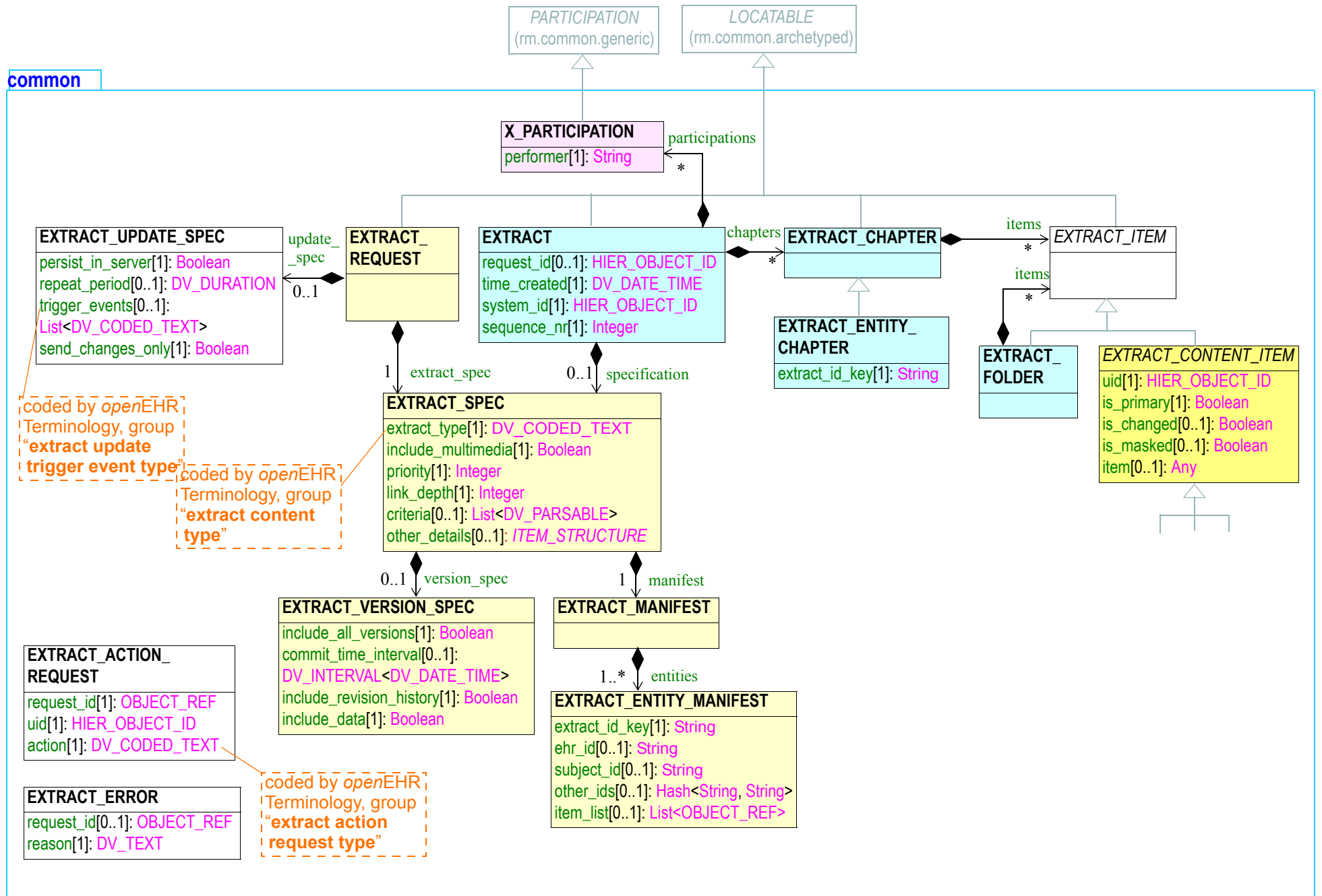
FIGURE 7 rm.extract.common Package
