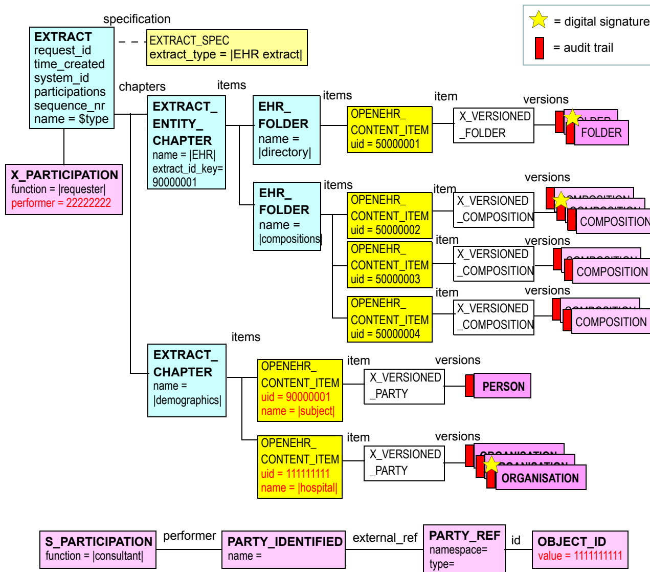
FIGURE 10 Typical EHR Extract structure
