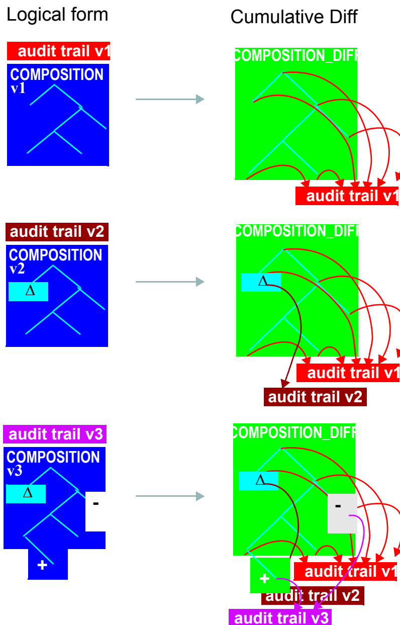
FIGURE 17 Generation of Cumulative Difference Form
