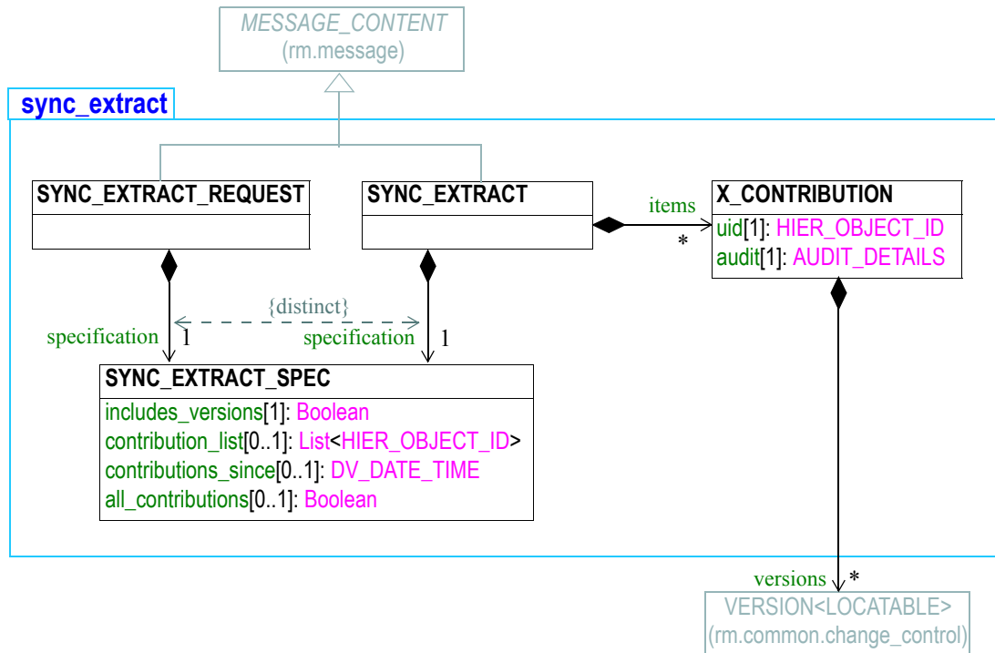
FIGURE 13 rm.extract.synchronisation_extract Package
