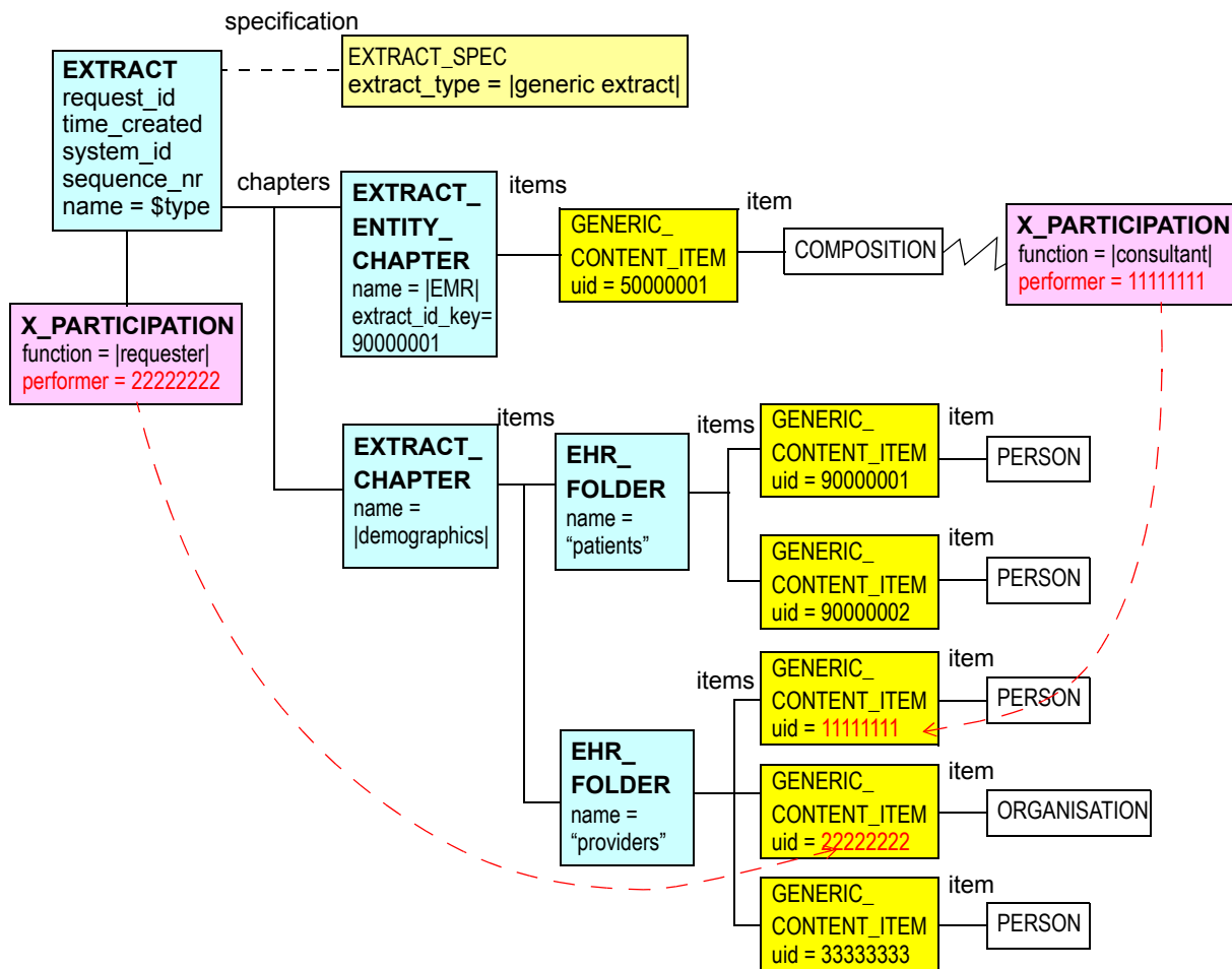
FIGURE 12 Typical generic extract structure
