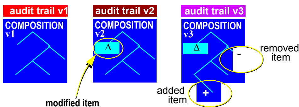
FIGURE 16 Successive Composition versions in a logical
